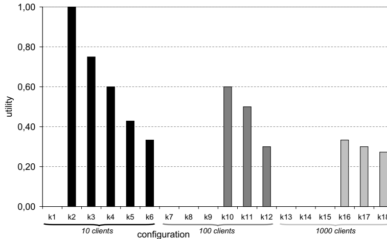
Figure 3: Utility function
