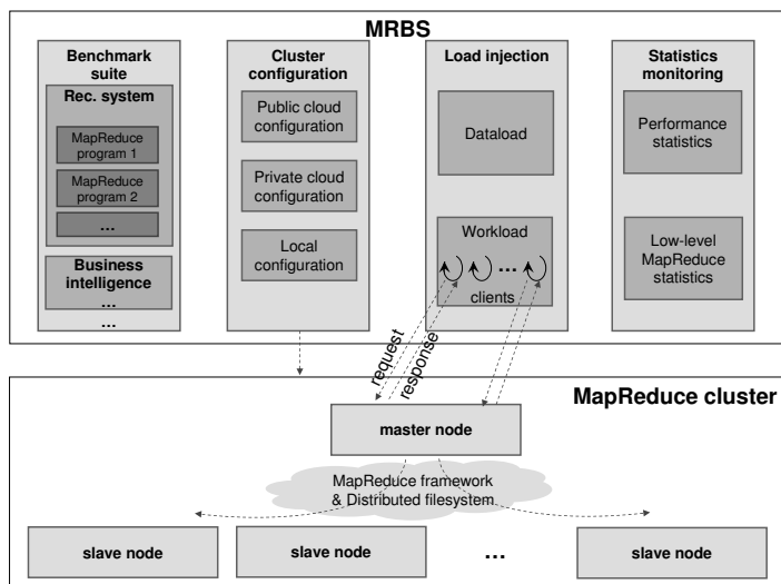
Figure 1. MRBS architecture
